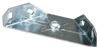
CORNER BRACKET A610 3/8" DIA THREAD, ZINC 1 1/3" H X 4" L
