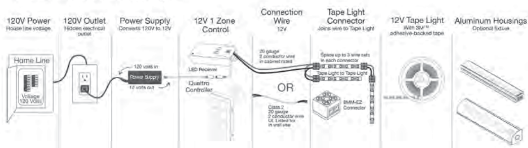
EXAMPLE – Basic Kit Hookup Diagram
